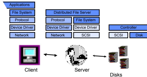
Figure 2 - Actual Distributed File System Architecture Today
