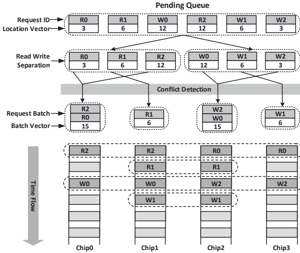
Figure 7. PIQ: RWS, RRS, and WWS are applied to the queue to separate the I/O requests into different batches based on the detected conflicts.
