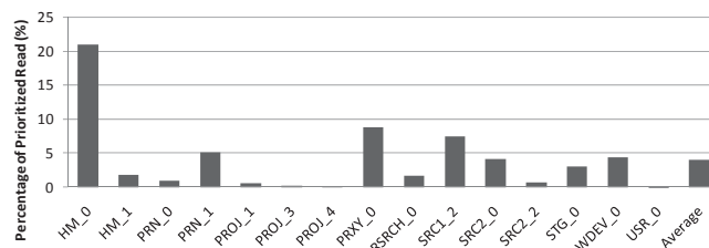
Figure 9. Percentages of prioritized read requests comparison between NOOP and RWS.
