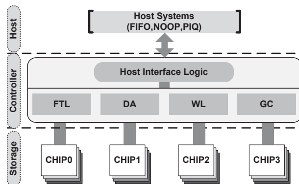
Figure 4. Organization of SSD based storage systems, where PIQ is implemented in host systems.
