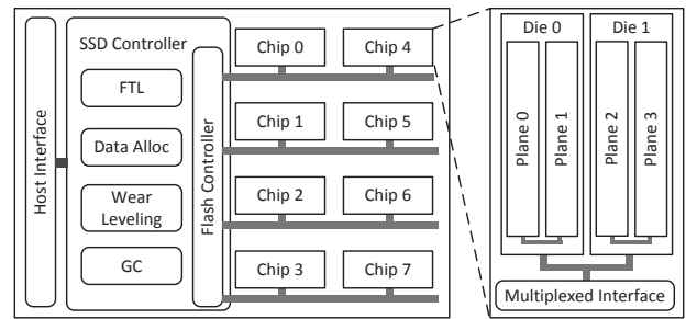
Figure 3. Architecture of SSD with four levels: Channels, Chips, Dies and Planes
