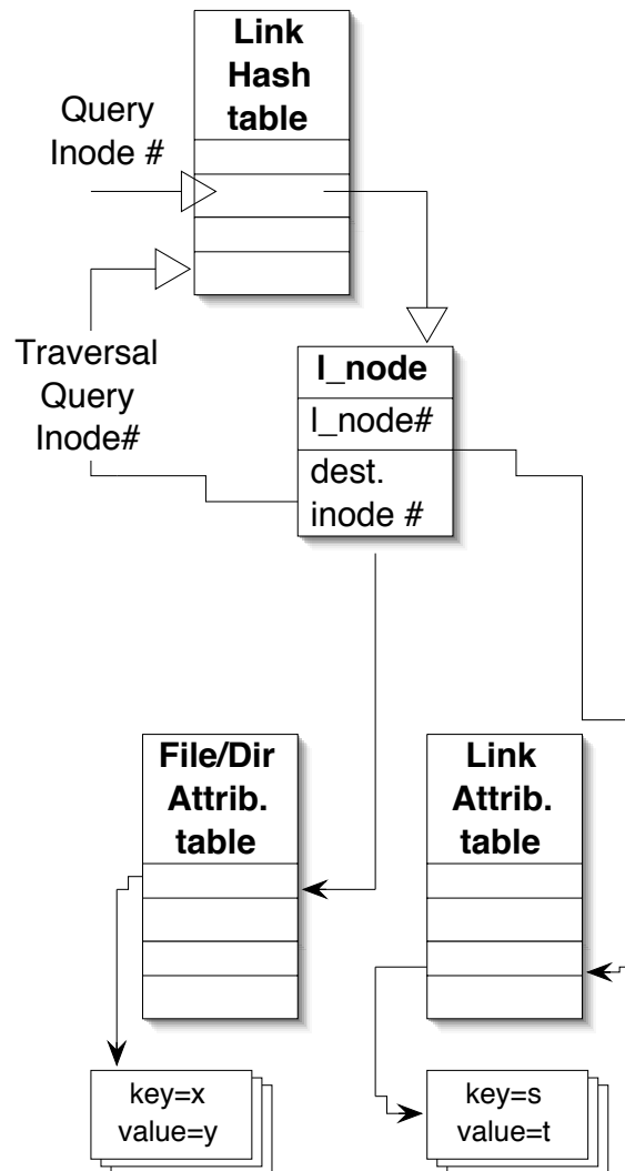
Figure 2. Hash tables to support links and attributes. A query returns links which can be iterated by attribute and can also seed a deeper traversal.
